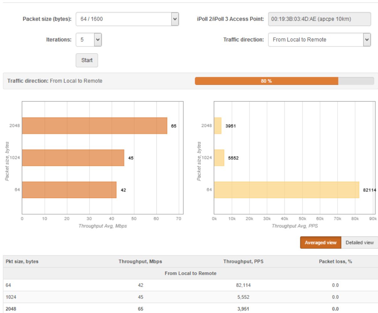
Figure 75 – Linktest Results
