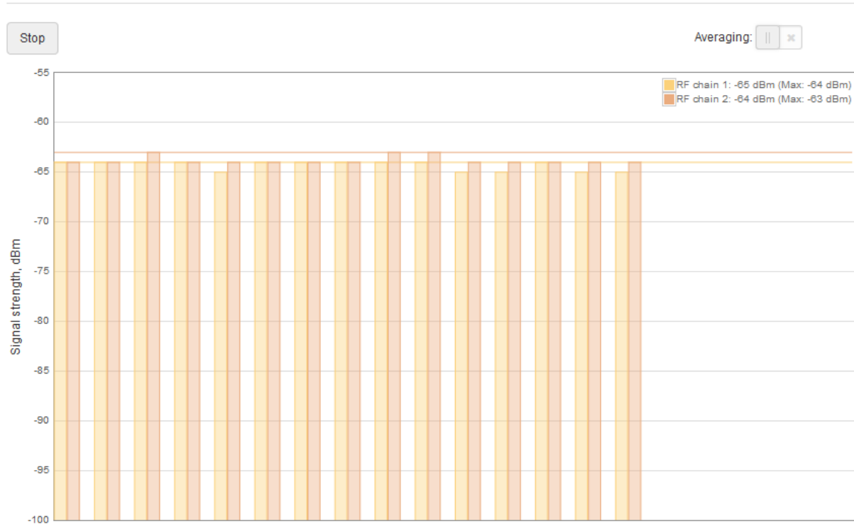
Figure 74 – Antenna Alignment
