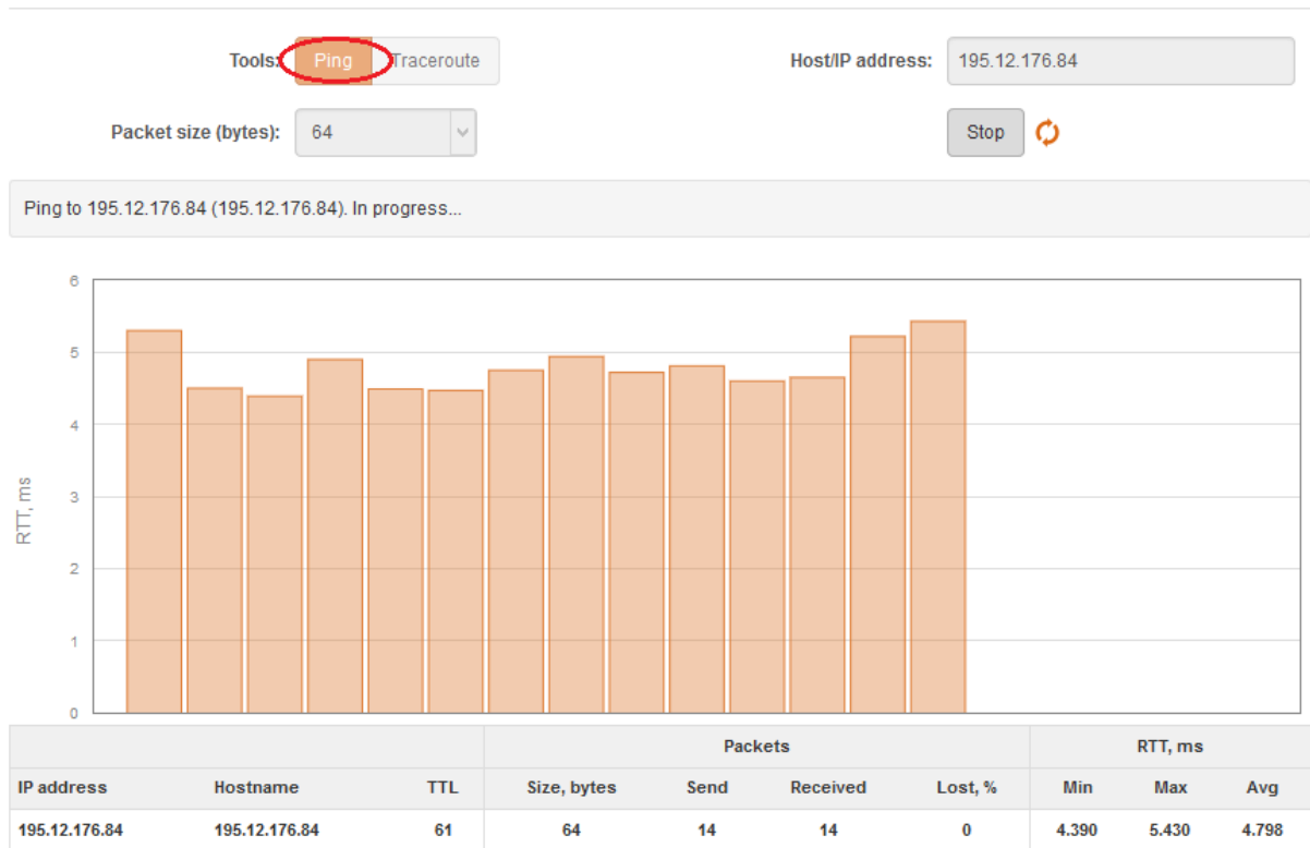
Figure 77 - Ping tool
